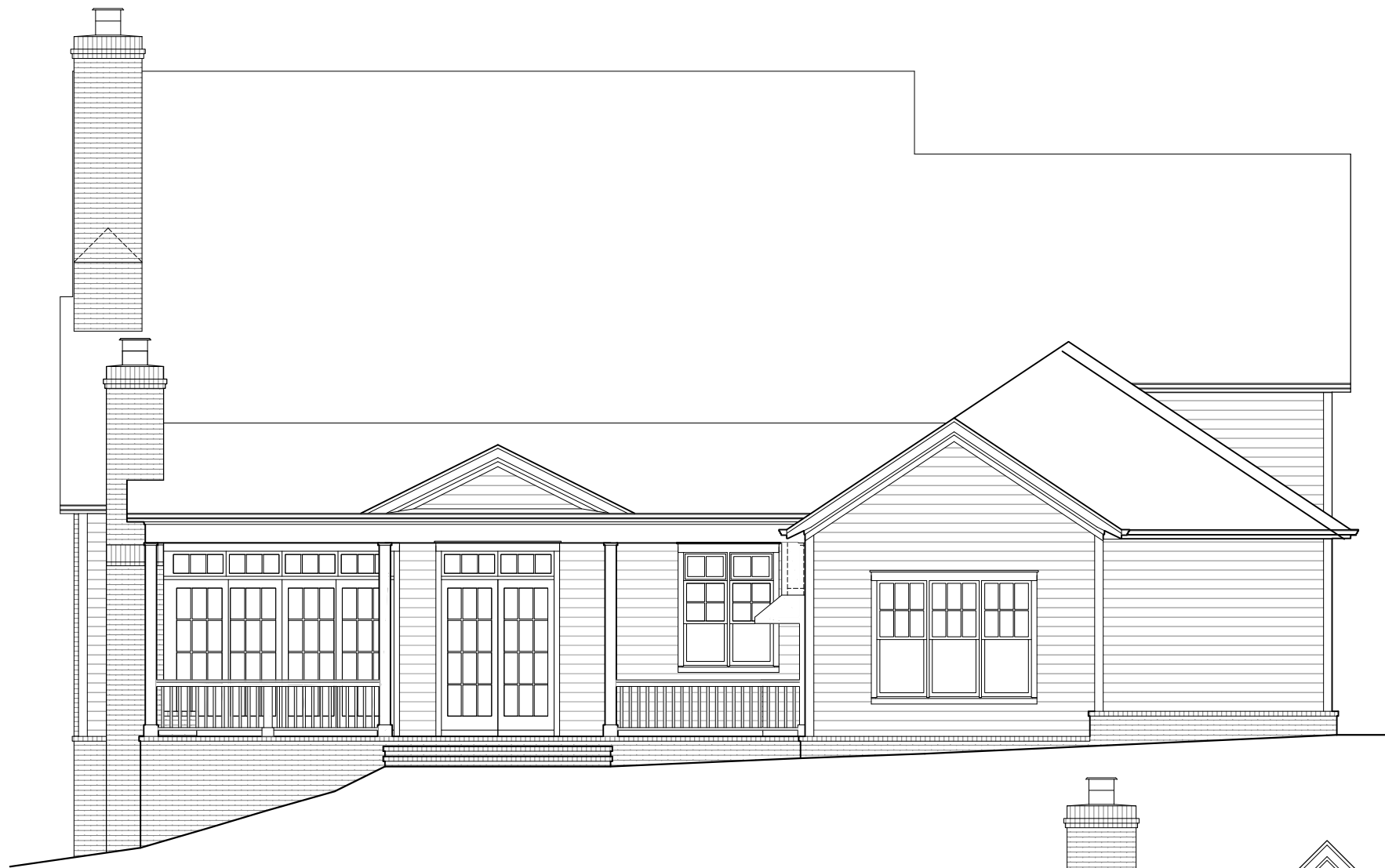
2 REAR ELEVATION 1/8" = 1'-0"
